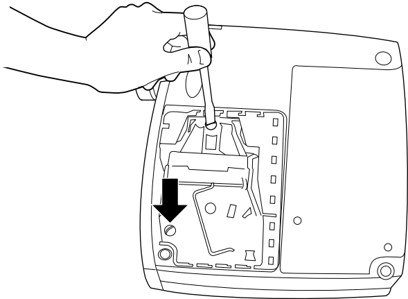
FIGURE 34 Loosening the screws on the lamp module
